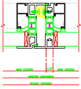
611 MEETING RAIL 325 P.L. | FIXED
