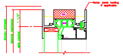
101 HEAD 325 FIXED | PROJECT IN
