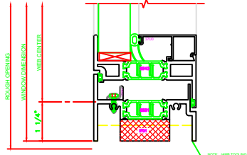
210 SILL 325 PROJECT IN 4-SWT ANGS
