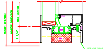
201 SILL 325 FIXED | CASEMENT IN
